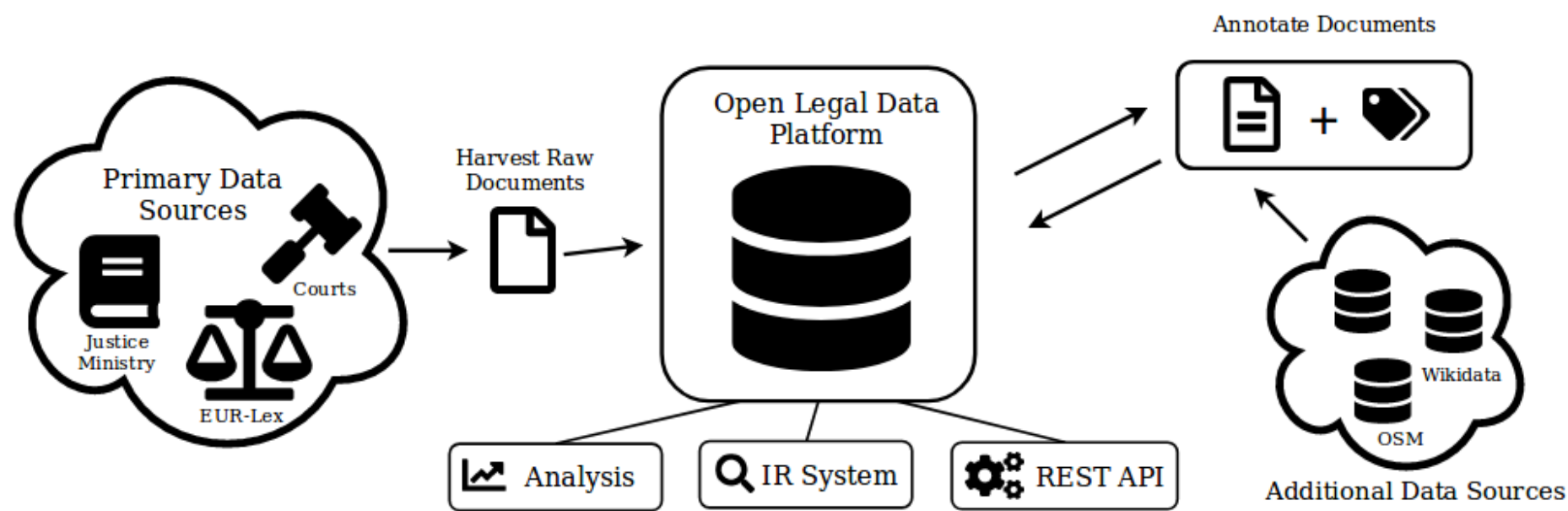
Figure 1: The OPENLEGALDATA.IO approach: Harvesting legal documents from official sources, extracting information from the raw documents and enriching the documents with data from additional sources. The platform content accessible through an API to facilitate analysis and retrieval tasks.
